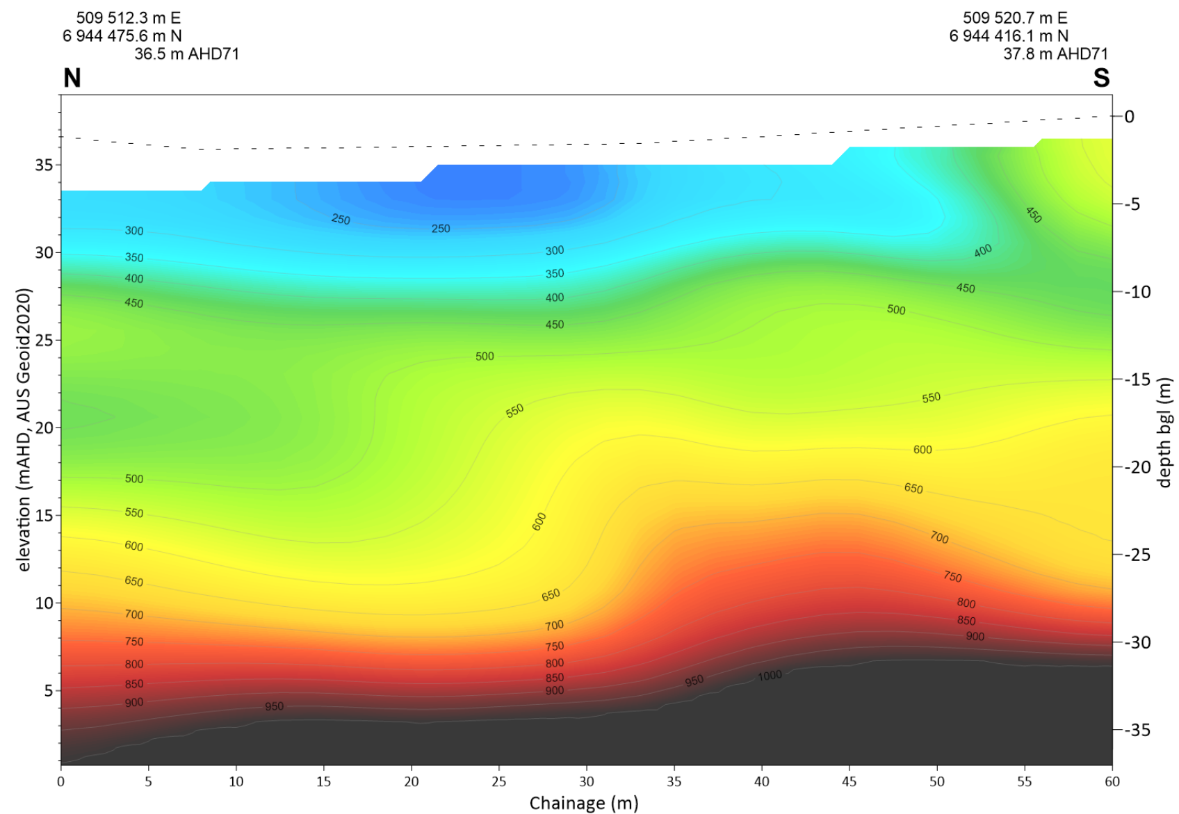
Seismic Line MASW AU-GP 117
